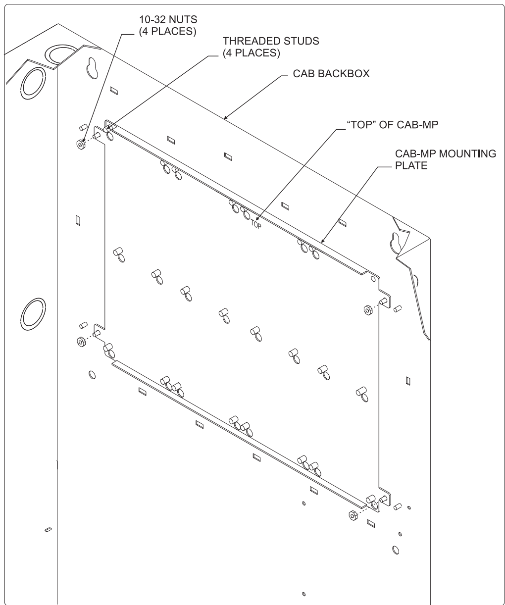
Figure 1 Installing The CAB-MP
