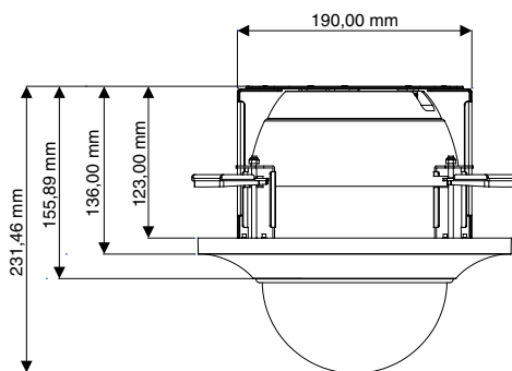
Using In-Ceiling Bracket
