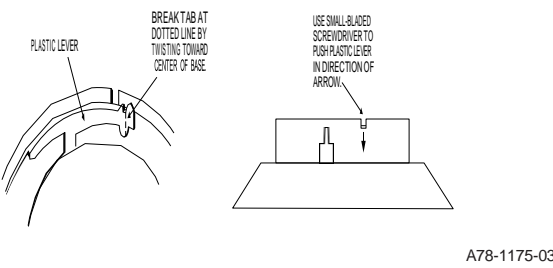
Figure 3B. Removing Detector Head from Base
