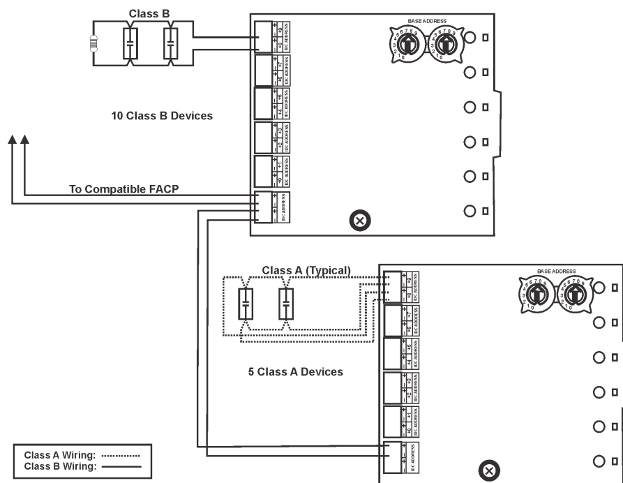
Wiring IDP-Monitor-10 Monitoring Modules
