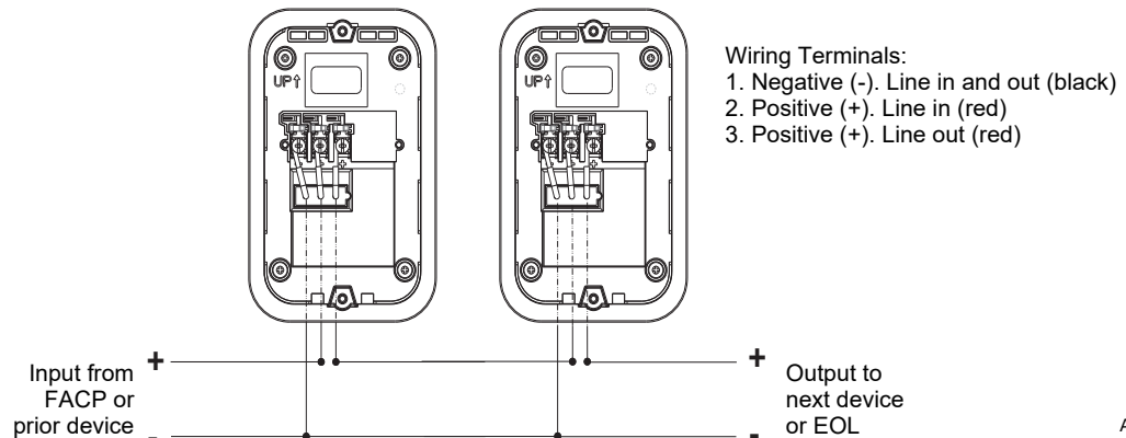
Figure 7 System Wiring
